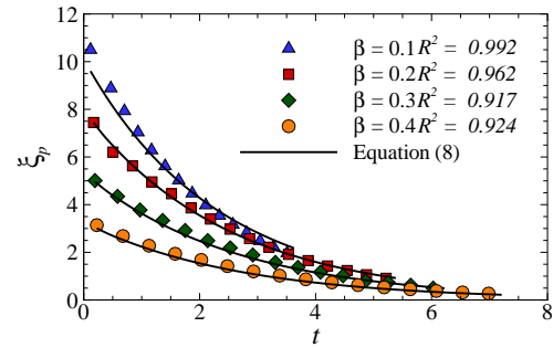
Figure 4. Decaying peak vorticity from numerical results and prediction by equation (8) for Ha = 250 and Re_L = 1500 . R^2 represents the quality of the curve fit.
