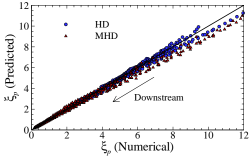
Figure 5. Overall comparison between numerical and predicted peak vorticity.
