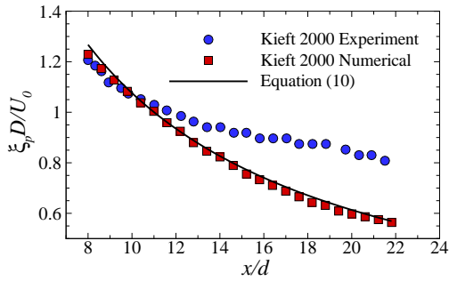
Figure 6. Comparison of predicted peak vorticity spatial evolution with the previous experimental data for Re_d = 75 .
