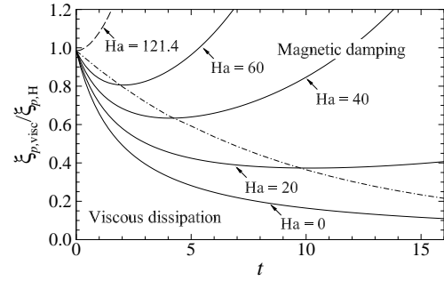
Figure 3. Time history of viscous-to-magnetic damping ratio for Re_L = 500 . Negative slope indicates region dominated by viscous dissipation and positive slope indicates region dominated by magnetic damping. Zero gradient indicates threshold of MHD dominated region. The dash-dotted line connects the turning point of each curve, separating two dominating regions and crosses y-axis at \xi_p(0) . The data is normalized by the initial peak vorticity.
