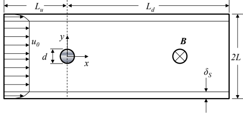
Figure 1. Schematic diagram of numerical domain. The shaded area indicates cylinder of infinite extension along the z -axis with diameter d .
