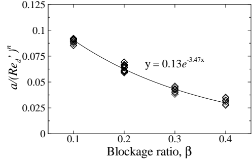
Figure 2. Curve fitting for constant a . In the curve-fit equation, y is a/(Re'_d)^{1.44} and x is the blockage ratio, \beta .
